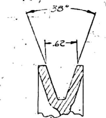
PULLEY FULL SIZE
